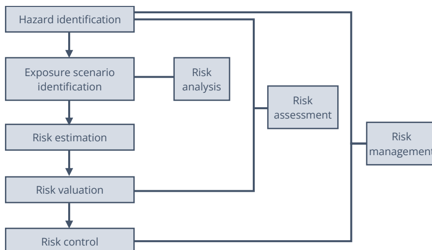
Fig. 8: Risk Management
