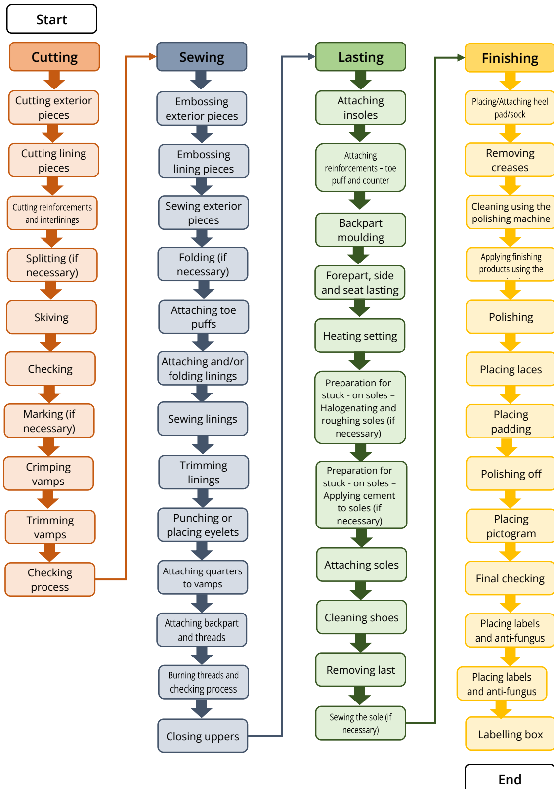
Fig. 9: Footwear production cycle - risk assessment
